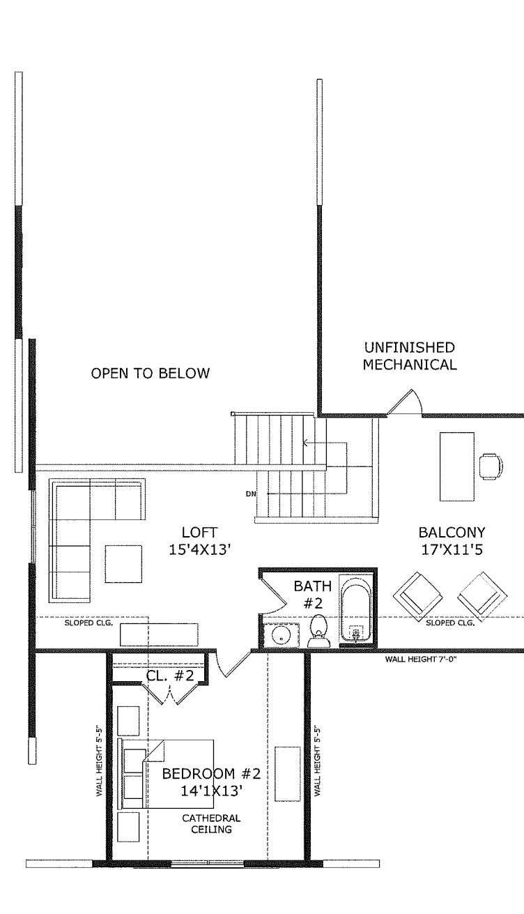
SECOND FLOOR - 696 S.F.
