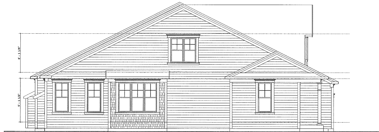
A-B Building LEFT SIDE
